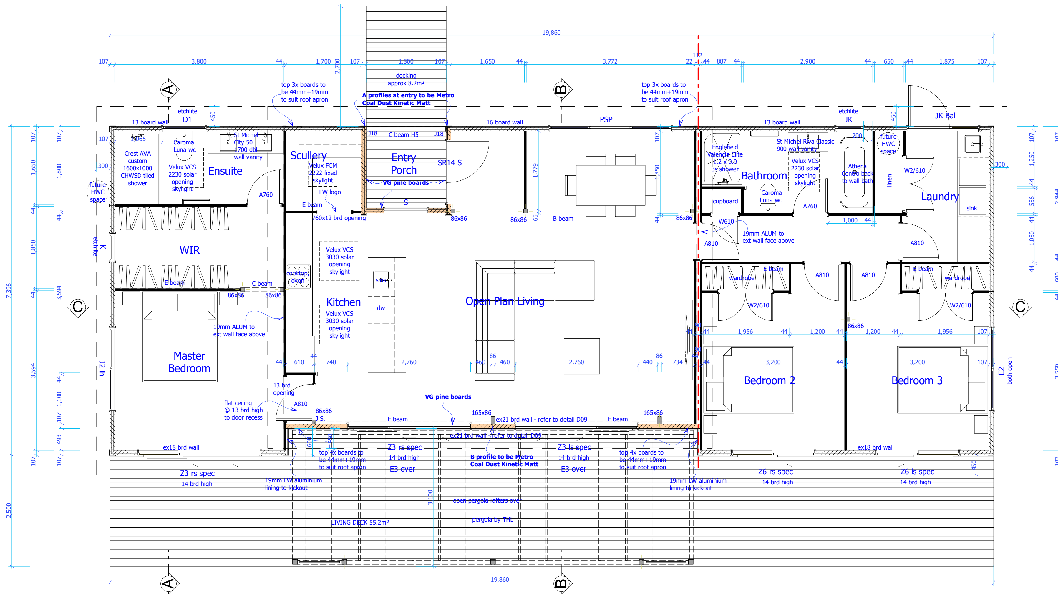
Floor Plan 1:50 Area = 137.96m 2
