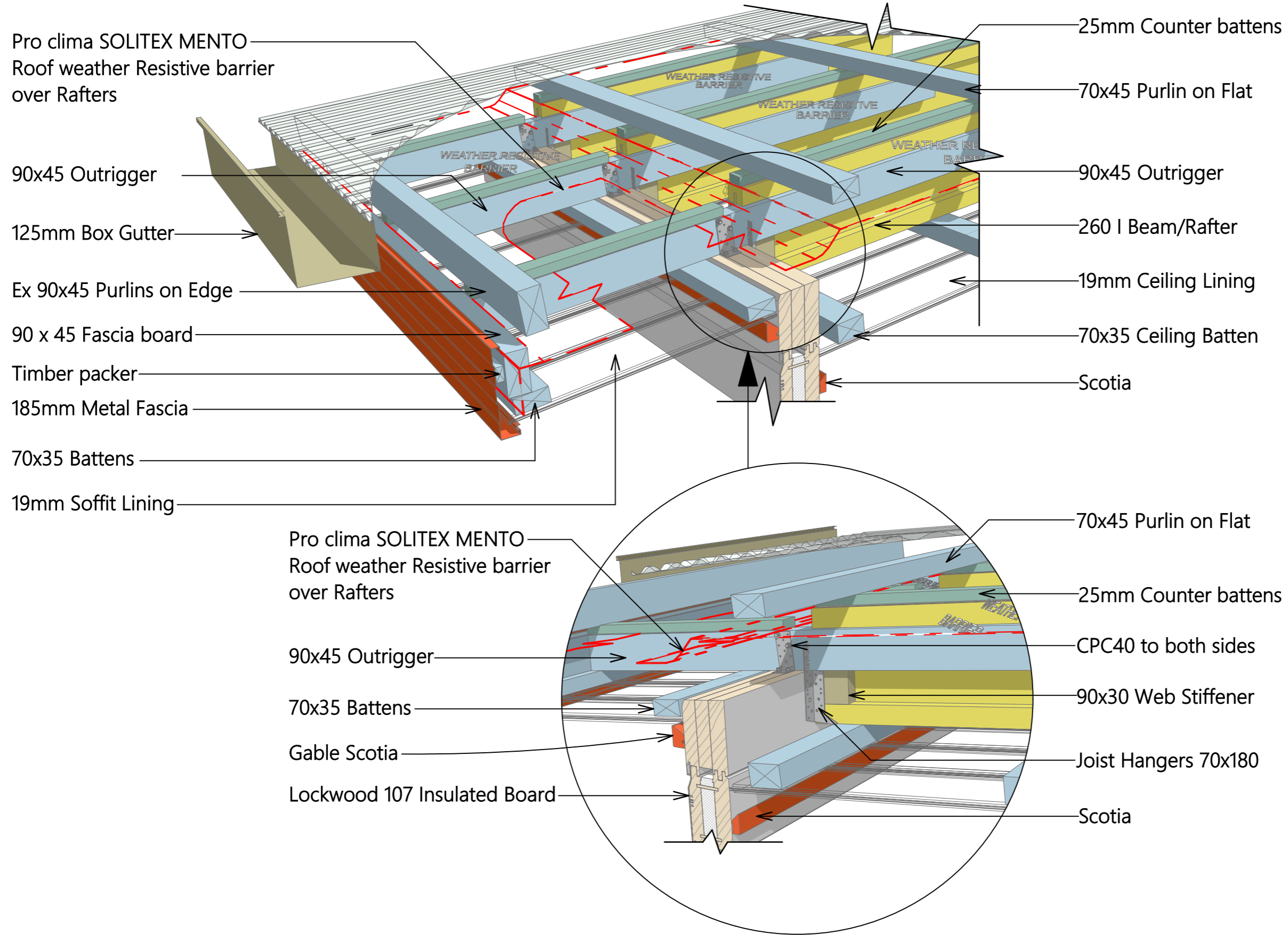
3D I-Rafter Soffit Detail
