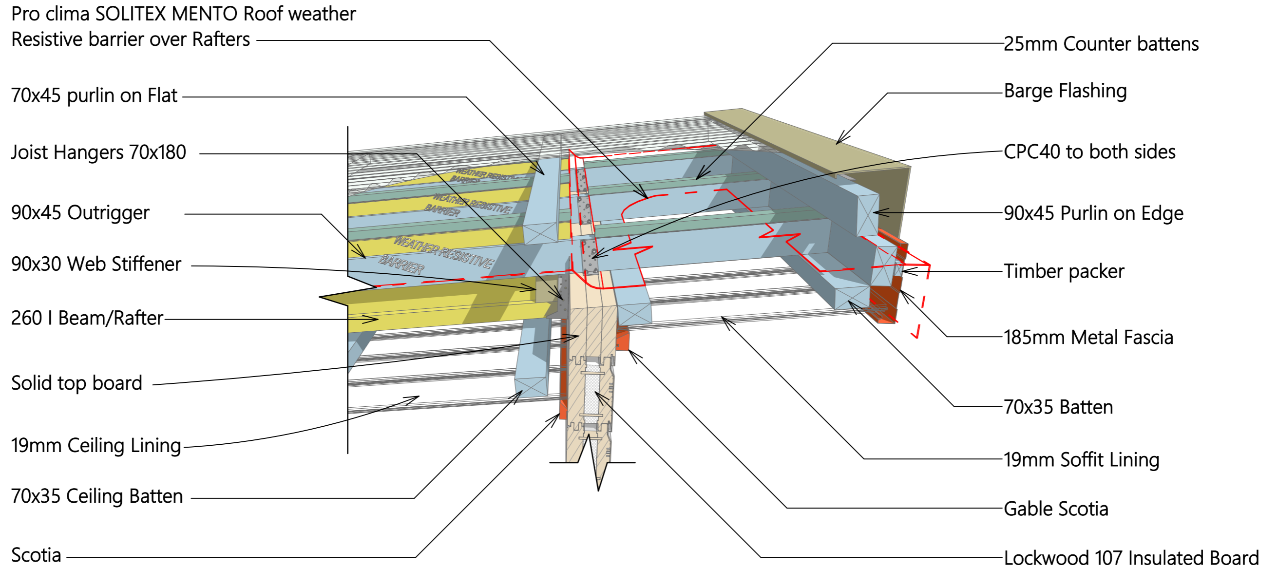
3D I-Rafter Raking Barge Detail
