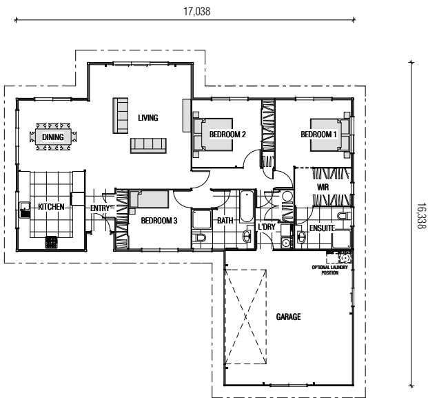
Rimu - three bedroom concept
