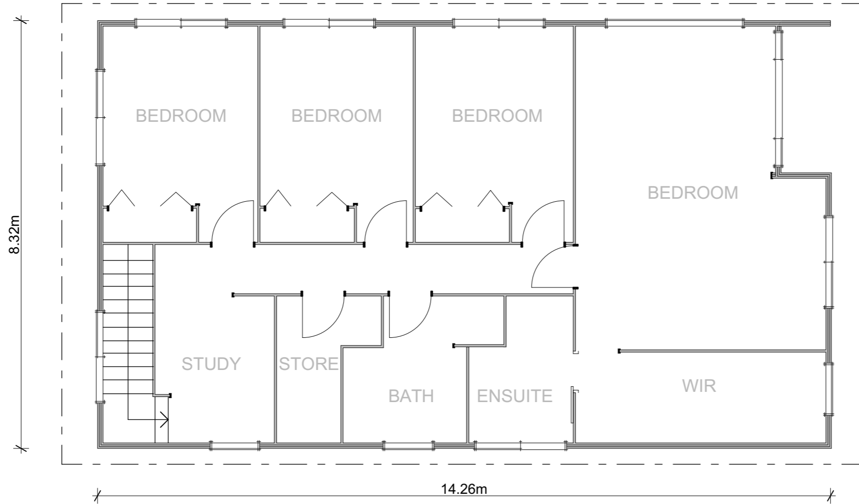
FIRST FLOOR
